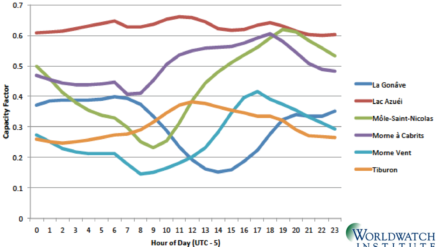
Diurnal Cycle of Capacity Factor at 80m
