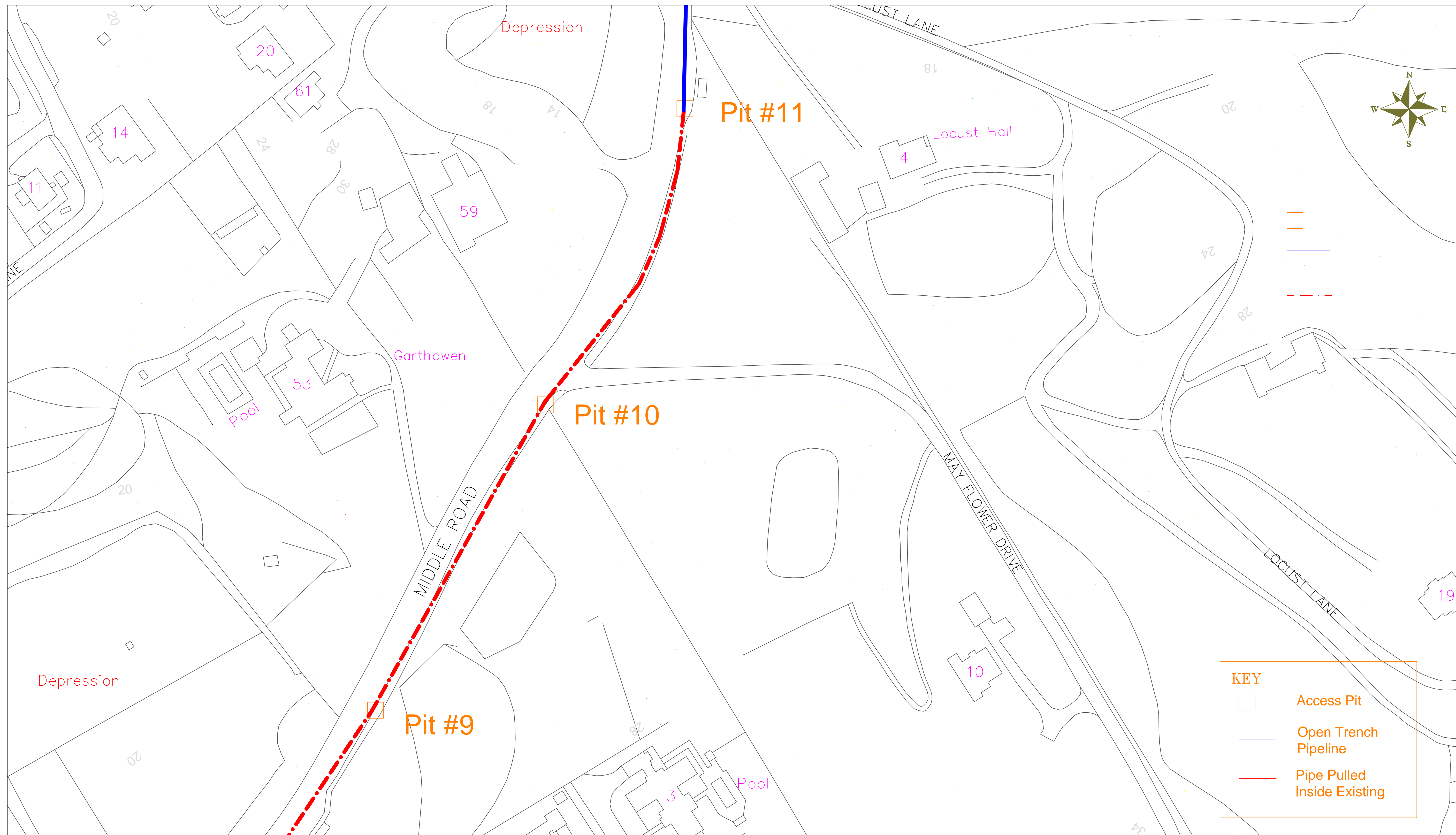
PIPELINE PLAN 1-500
